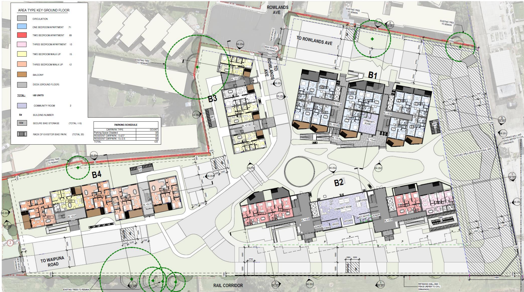
1 GROUND FLOOR PLAN SCALE 1 : 250
